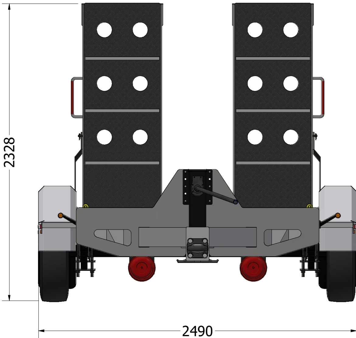
REAR VIEW
