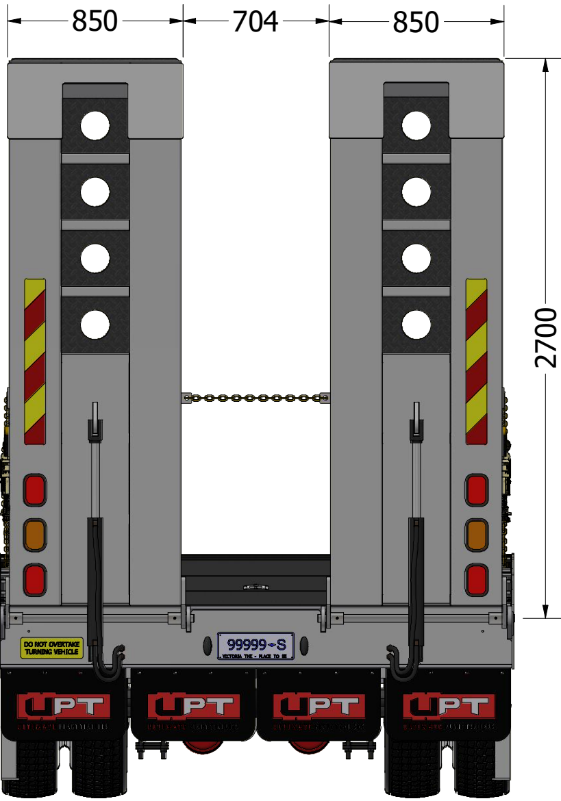
UPT 4-AXLE DOG
