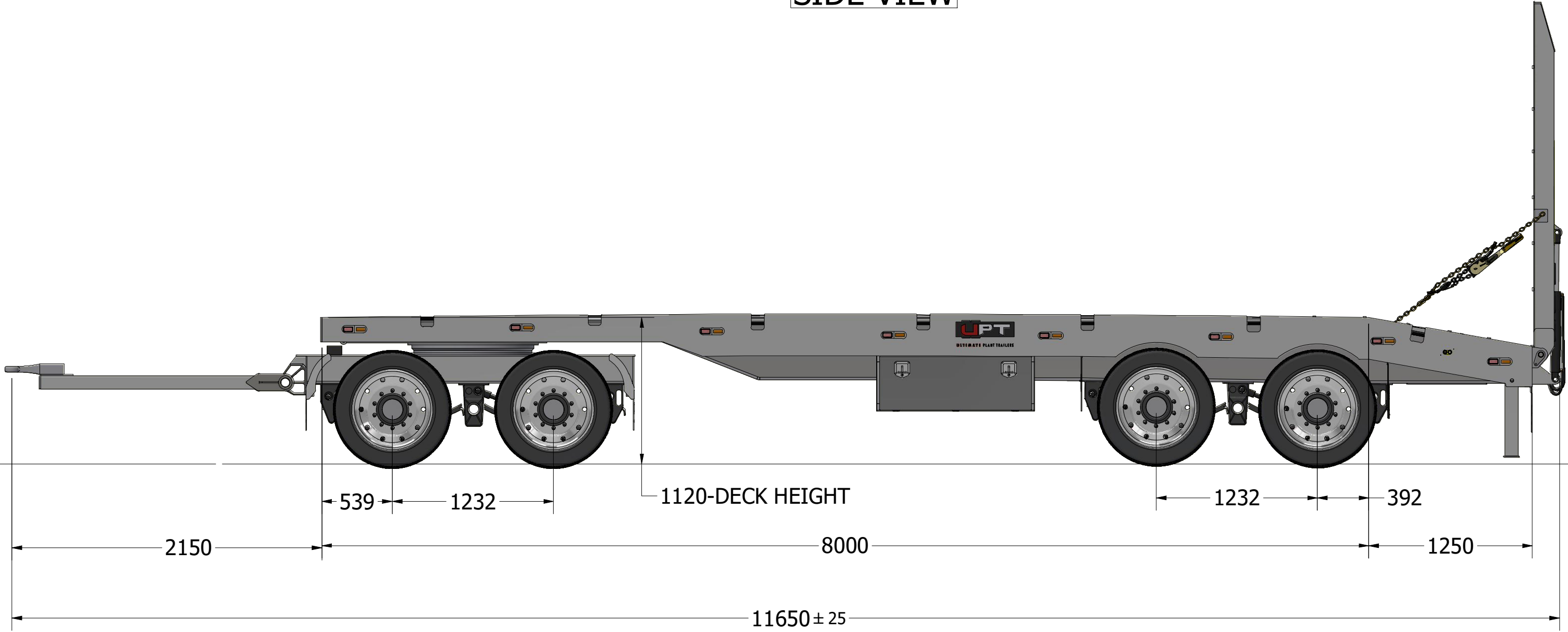
SIDE VIEW
