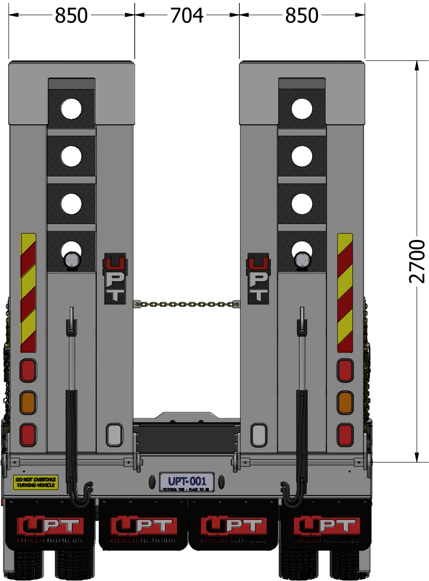
UPT TANDEM AXLE
