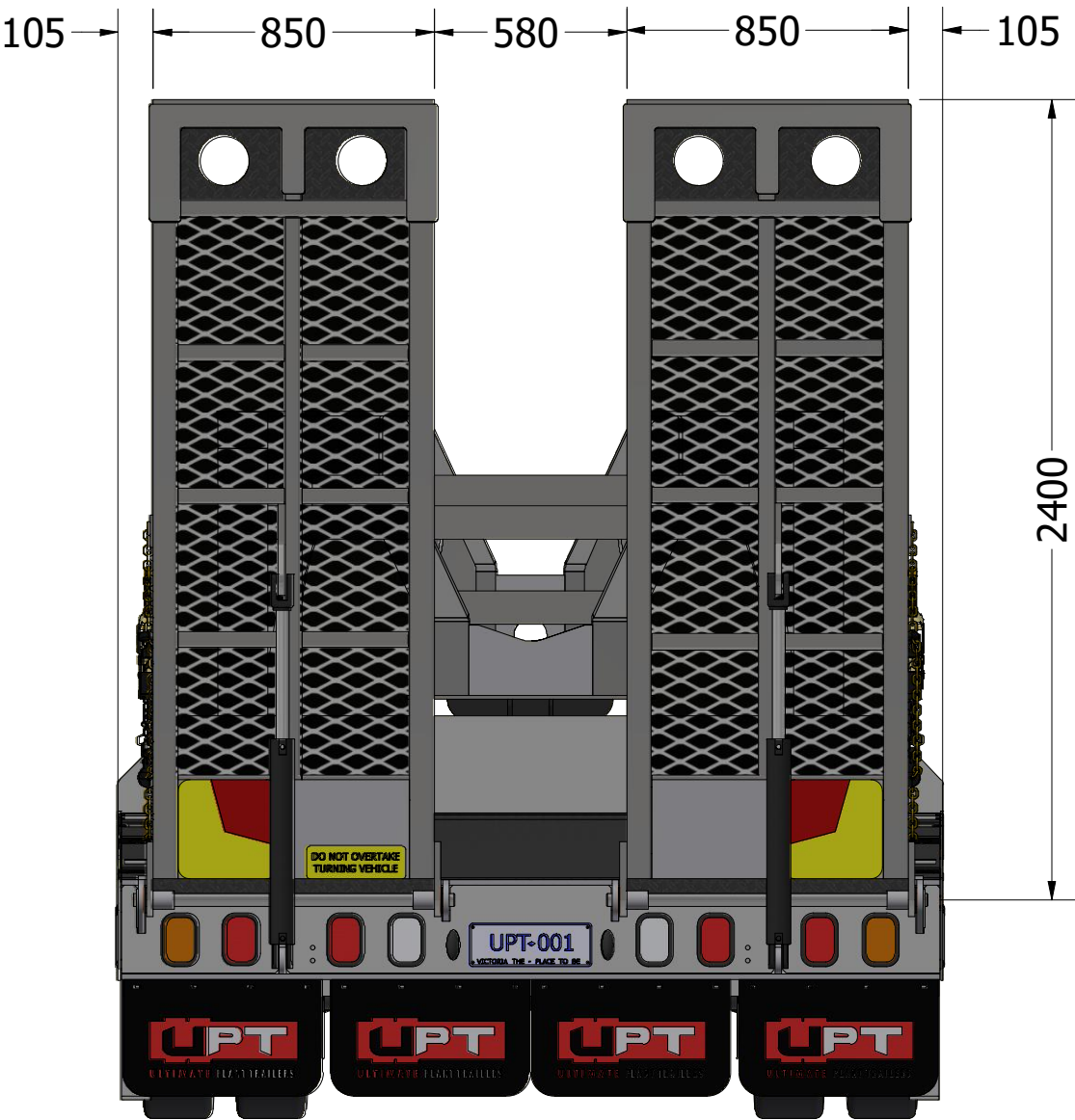
REAR VIEW
