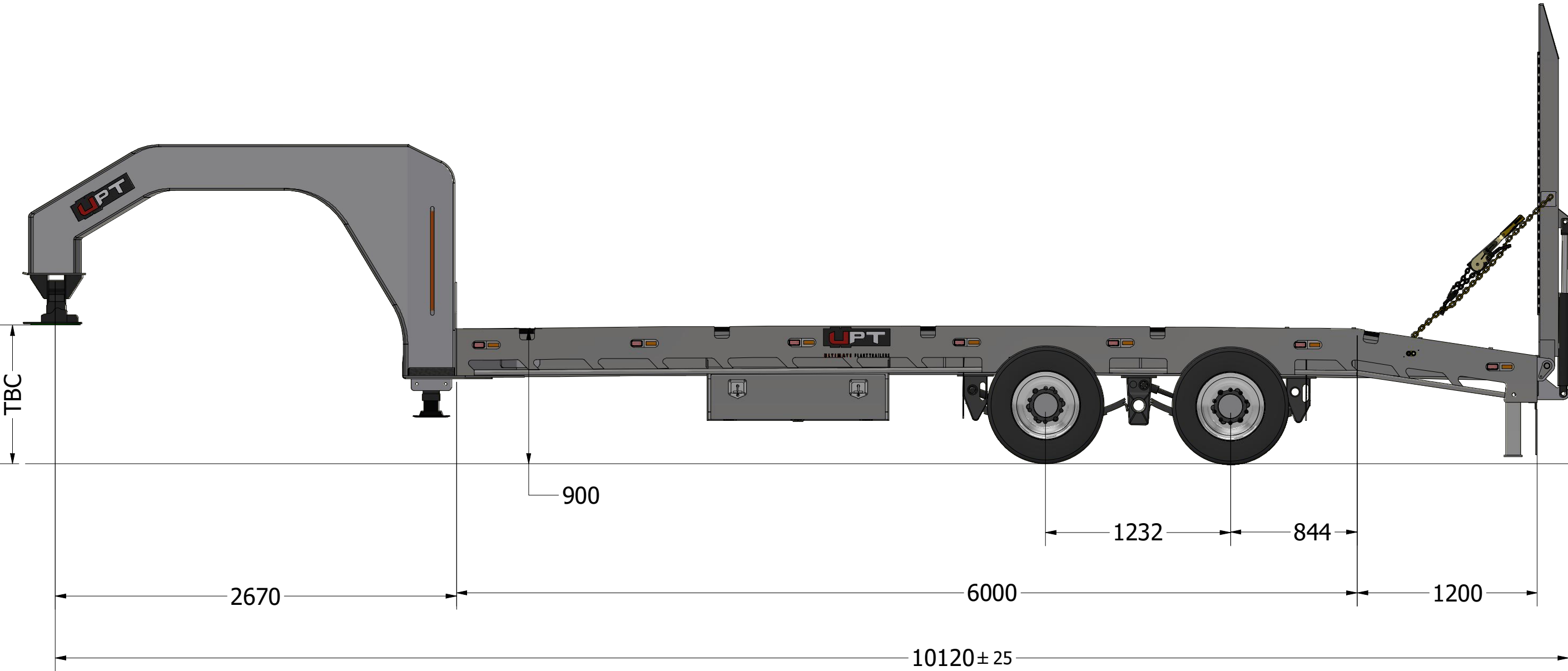
SIDE VIEW
